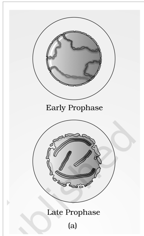
Fig. 10.2 (a) - A diagrammatic view of stages in mitosis: early prophase and late prophase.
