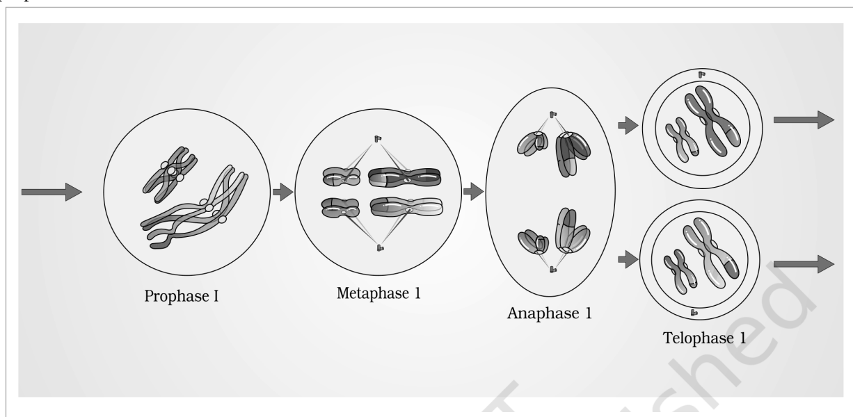
Fig. 10.3 - Stages of Meiosis I.
