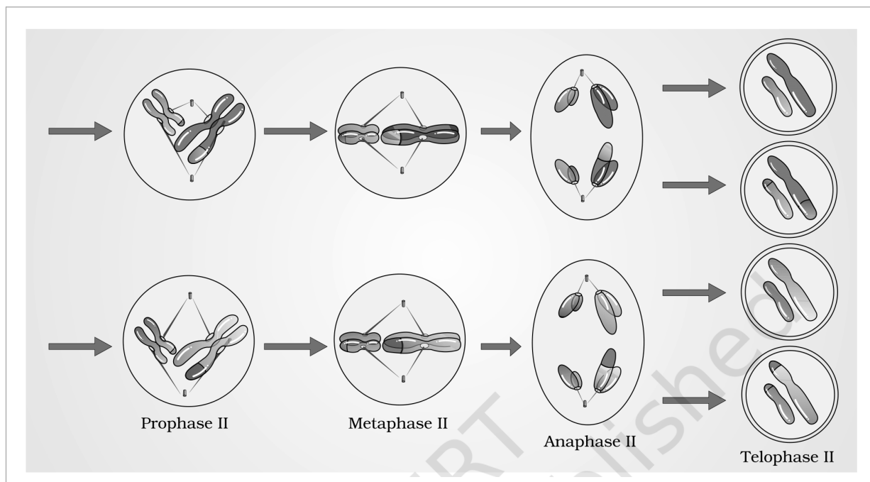
Fig. 10.4 - Stages of Meiosis II.
