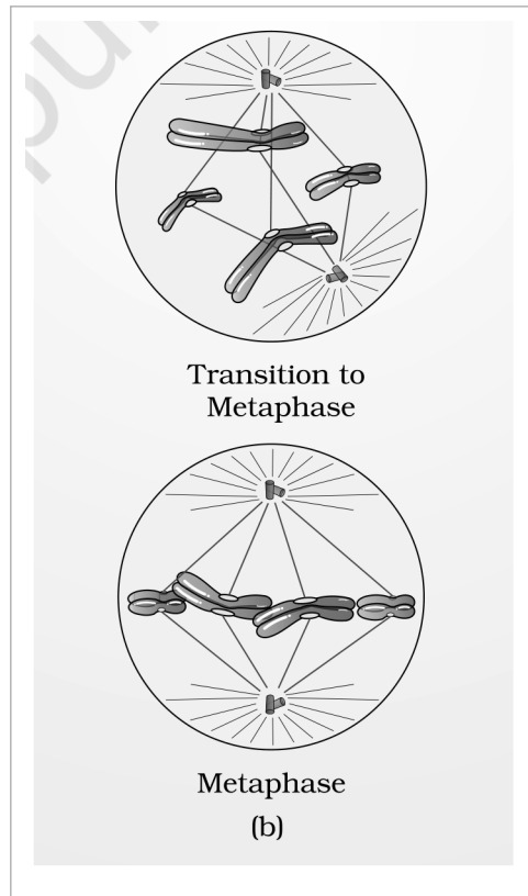
Fig. 10.2 (b) - A diagrammatic view of stages in mitosis: transition to metaphase and metaphase.
